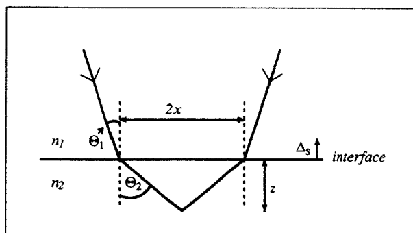
Fig. 1. Geometry of the system. A convergent light wave which travels through a medium with refractive index n_1 is focused in a second medium with refractive index n_2 . Indicated is the normal to the interface (dashed). The marginal rays make an angle \theta_1 with the normal before refraction, and an angle \theta_2 after refraction. In this example n_1 > n_2 .
