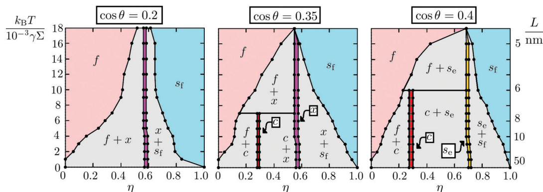
Fig. 9 Temperature–density phase diagram for \cos \theta \in \{0.2, 0.35, 0.4\} . The left vertical axis is the dimensionless temperature k_{\text{B}} T / (10^{-3} \gamma \Sigma) , with \gamma the fluid–fluid surface tension, \Sigma the total surface area of a particle, k_{\text{B}} the Boltzmann constant, and T the temperature. The right vertical axis represents the corresponding value of the particle size L at room temperature (300 K) and using a typical surface tension \gamma = 0.01 \text{ N m}^{-1} . The horizontal axis is the particle density \eta , which is equal to 1 for the close-packed “face up” square phase s_f . The colored areas indicate stable 2D one-phase regions at the fluid–fluid interface: light-pink indicates a disordered fluid phase f , while red, magenta, yellow, and light-blue the chains c , hexagonal x , “edge up” square s_e , and “face up” square s_f phases, respectively. The gray areas indicate coexistence between two phases of different \eta , and the horizontal lines connect three phases coexisting at the f – c – x , and f – c – s_e triple points, respectively.
